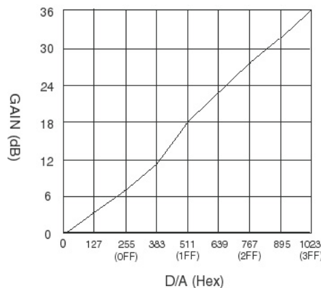
Figure 8. Camera Gain Curve
