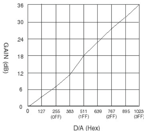
Figure 9. Camera Gain Curve
